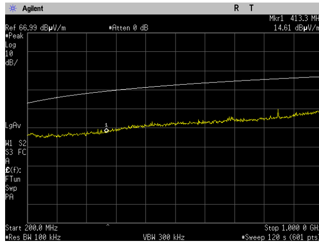
Plot 1.10: RE102 test results within 200 – 1000 MHz, horizontal polarization
