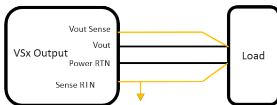
Figure 3 – Sense Lines connection
