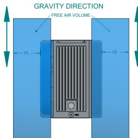
SUGGESTED KEEP OUT AREA FOR NATURAL CONVECTION
