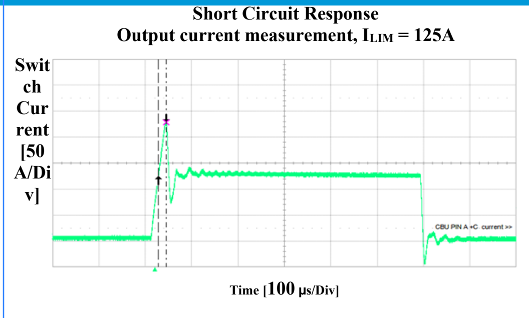
Figure 2 - Short Circuit Response
